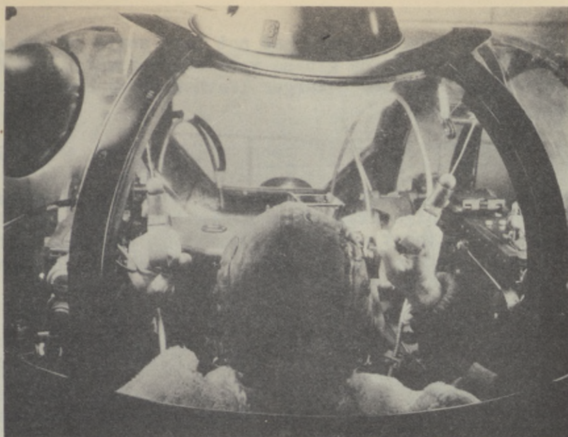
CHARGING GUNS
