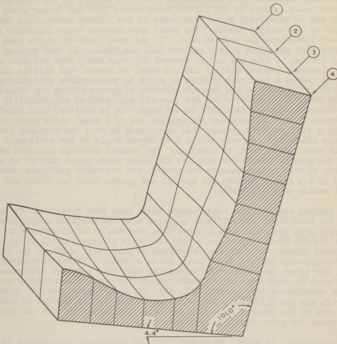
SEAT SECTION FOR 45" BOMBER COCKPIT, SHOWING PROFILES AT \frac{1}{2} (4) AND AT THREE INCH INTERVALS Laterally (3) - (2) & (1).
