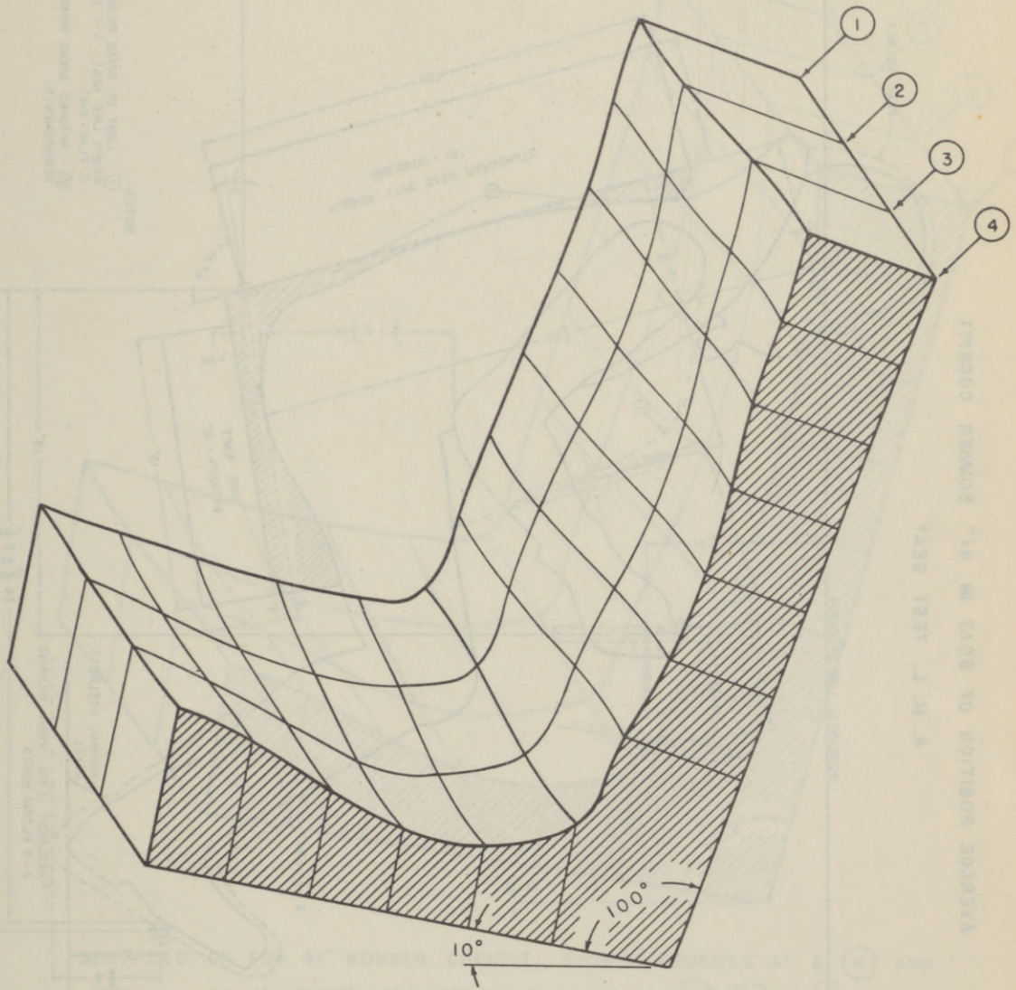
SEAT SECTION FOR 39" BOMBER COCKPIT, SHOWING PROFILES AT \phi (4) AND AT 4477-C. A.M.L. THREE INCH INTERVALS Laterally (3) - (2) & (1).
