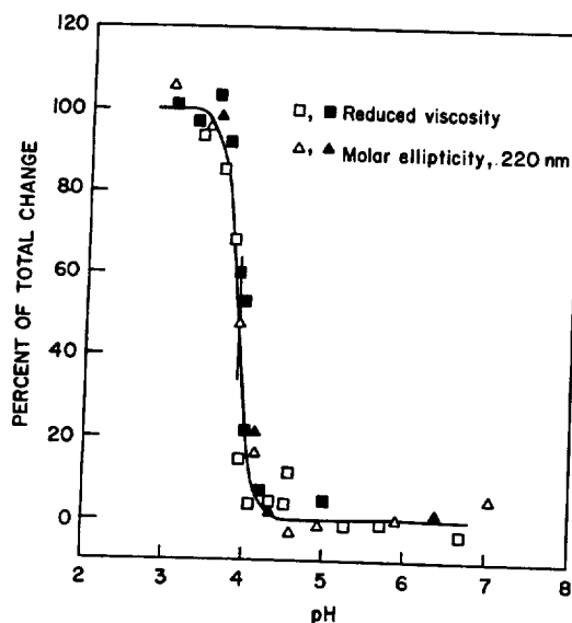
Fig. 9. Changes in reduced viscosity and molar ellipticity at 220 nm during the acid-induced transition from native to denatured nuclease.
