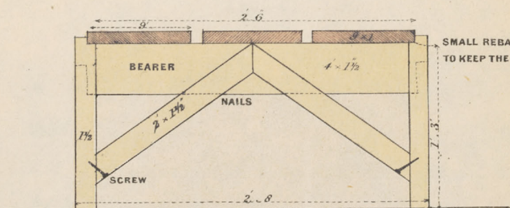
END VIEW
