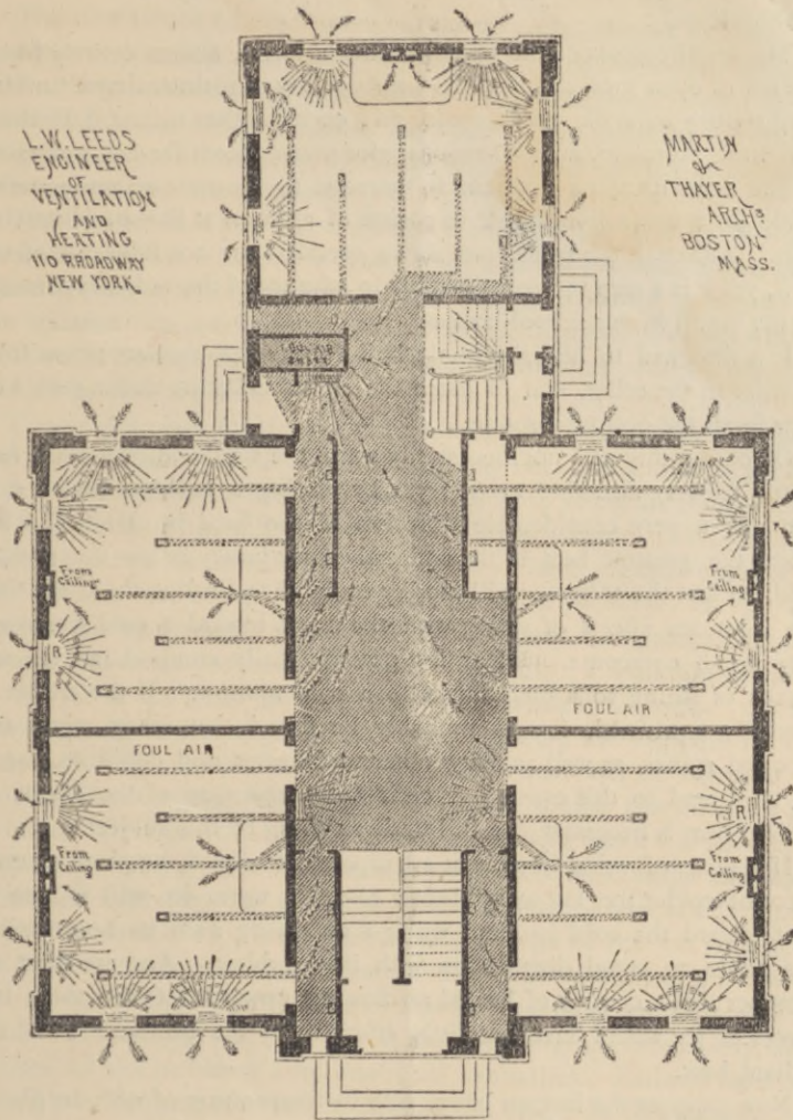
PLAN OF SALEM SCHOOL-HOUSE, FIRST FLOOR.
