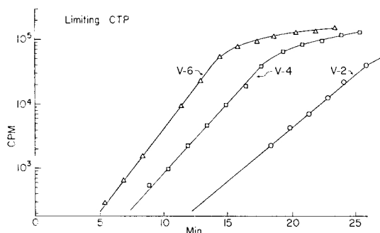
FIG. 2.—Synthesis of variants on a reaction mixture with a limiting CTP concentration. A reaction mixture containing only 1 m\mu mole (instead of 100 m\mu moles) CTP, including 2.2 \times 10^5 cpm H^3 -CTP, was incubated at 38°C with 40 \mu g Q \beta -replicase and 0.001 \mu g of purified V-2, V-4, or V-6 RNA. The amount of trichloroacetic acid-insoluble radioactive material was determined at the indicated times. In this experiment 1.7 \times 10^6 cpm is equivalent to 1 \mu g of variant RNA.
