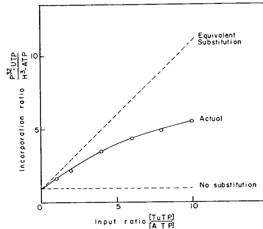
FIG. 4.—Substitution of ATP by TuTP. Synthesis of RNA templated by 0.001 \mu\text{g} V-8 RNA in the presence of 40 \mu\text{g} Q \beta -replicase was allowed to take place for 40 min in a reaction mixture containing 5 \mu\text{moles} ATP, the indicated amounts of TuTP, and H 3 -ATP and P 32 -UTP. The U to A ratio in plus strands of variant is 6/5, which we may take as unity. If tubercidin can replace adenosine with equal probability, the U to A ratio in the product should vary with the ratio of TuTP to ATP in the reaction mixture in the manner described by the upper dashed curve (labeled equivalent substitution ). If there is no substitution of adenosine by tubercidin, the ratio of U to A should remain normal and independent of the relative amounts of TuTP present (lower dashed curve labeled no substitution ). The unbroken line indicates the actual incorporation ratio corrected for an input of 6 \times 10^5 cpm/100 \mu\text{moles} P 32 -UTP and 5 \times 10^5 cpm/100 \mu\text{moles} H 3 -ATP.
