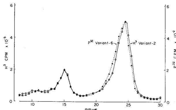
FIG. 3.—Gel electrophoresis of V-2 and V-6. Standard reaction mixtures of 0.0125 ml initiated with 0.001 \mu g of V-2 in the presence of 2.2 \times 10^6 cpm H^3 -UTP, or 0.001 \mu g of V-6 in the presence of 2 \times 10^6 cpm P^{32} -UTP were incubated for 18 and 13 min, respectively. The reactions were terminated with 0.01 ml 2.5% sodium dodecyl sulfate and mixed together. The mixture was electrophoresed through polyacrylamide gels and processed as in Materials and Methods .
