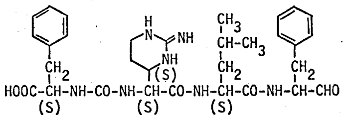
Chymostatin
