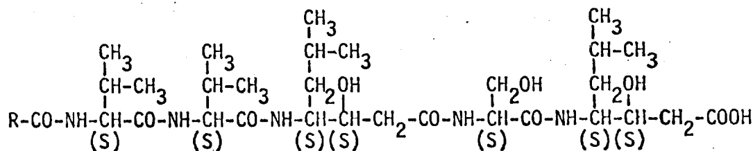
Hydroxy pepstatin
