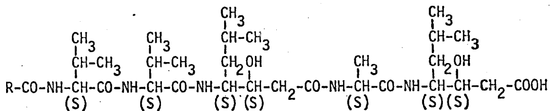
Pepstatin
