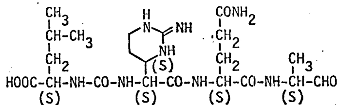
Elastatinal
