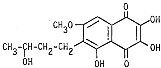
6-(3-hydroxy-n-butyl)-7-O- methylspinochrome B inhibiting catechol-O- methyltransferase
