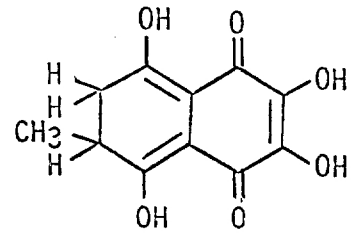
Dihydromethylspinazarin inhibiting catechol-O- methyltransferase
