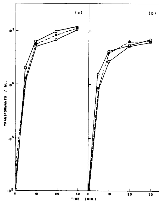
FIG. 3. Effect of the addition of poly-dCdG and poly-dAdT on transformation. Experimental conditions as in Table 1 except that the concentration of transforming DNA was 0.1 \mu\text{g}/\text{ml} of cell suspension. At the shown time intervals, 0.1 ml of cell suspension was pipetted into 0.4 ml of Spizizen medium containing 10^{-2} M \text{Mg}^{++} and 5 \mu\text{g} of deoxyribonuclease per ml, and incubated for 10 min at 37 C. Tryptophan transformants were scored. (a) ●, DNA at 0.1 \mu\text{g}/\text{ml} ; ○, 0.1 \mu\text{g} of DNA plus 0.1 \mu\text{g} of poly-dAdT per ml; □, 0.1 \mu\text{g} of DNA plus 1 \mu\text{g} of poly-dAdT per ml. (b) Same as (a) except that poly-dCdG was used in place of poly-dAdT.
