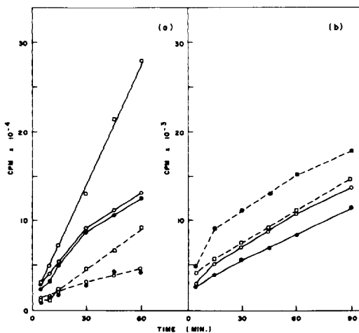
FIG. 2. Stimulation of ^{14}\text{C} -amino acid incorporation in the presence of synthetic polyribonucleotides. (a) Solid lines, ^{14}\text{C} -phenylalanine (1.5 \mu\text{Ci/ml} ); dashed lines, ^{14}\text{C} -lysine (1.5 \mu\text{Ci/ml} ) were added to competent cells previously washed and suspended in Spizizen minimal medium (10) containing 0.5% glucose. The trichloroacetic acid-insoluble counts were determined on 0.2-ml samples of cell suspension withdrawn at the time intervals indicated. \circ , No addition; \bullet , plus 100 \mu\text{g} of poly-rA per ml; \square , plus 100 \mu\text{g} of poly-rU per ml. (b) Dashed lines, ^{14}\text{C} -phenylalanine (0.25 \mu\text{Ci/ml} ) as in (a) in the presence ( \blacksquare ) or in the absence ( \square ) of 100 \mu\text{Ci} of poly-rUrA per ml; solid line, ^{14}\text{C} -arginine (0.25 \mu\text{Ci/ml} ) in the presence ( \circ ) or in the absence ( \bullet ) of 100 \mu\text{g} of poly-rUrA per ml.
