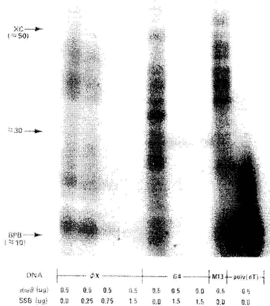
FIG. 2. Electrophoresis of RNA primer transcripts. Reaction mixtures (25 \mu l) contained: 5 \mu l of buffer A; 0.2 \mu mol of MgCl_2 ; 1.25 nmol each of [ \alpha - ^{32}P ]GTP, CTP, and UTP (each at 7000 dpm/pmol); 20 nmol of ATP; 0.1 \mu g of rifampicin; 500 pmol (as nucleotide) of phage DNA; 0.15 \mu g of primase; and additional components as indicated. The poly(dT) reaction mixture contained [ \alpha - ^{32}P ]ATP (1000 dpm/pmol) and 4 nmol of poly(dT). Incubation was at 30°C for 30 min. The reaction was terminated by cooling to 0°C. To each sample were added 50 \mu l of 95% ethanol (-20°C), 2.5 \mu l of 3 M sodium acetate (pH 5.5), and 30 \mu g (1 \mu l) of E. coli tRNA. After 4 hr at -20°C, the precipitates were collected by centrifugation and resuspended in 25 \mu l of deionized formamide. RNA transcripts were fractionated by electrophoresis in a 15% polyacrylamide gel containing 7 M urea and located by autoradiography (20, 21). Approximate lengths are given on the left in nucleotides. XC, xylene cyanol; BPB, bromphenol blue.
